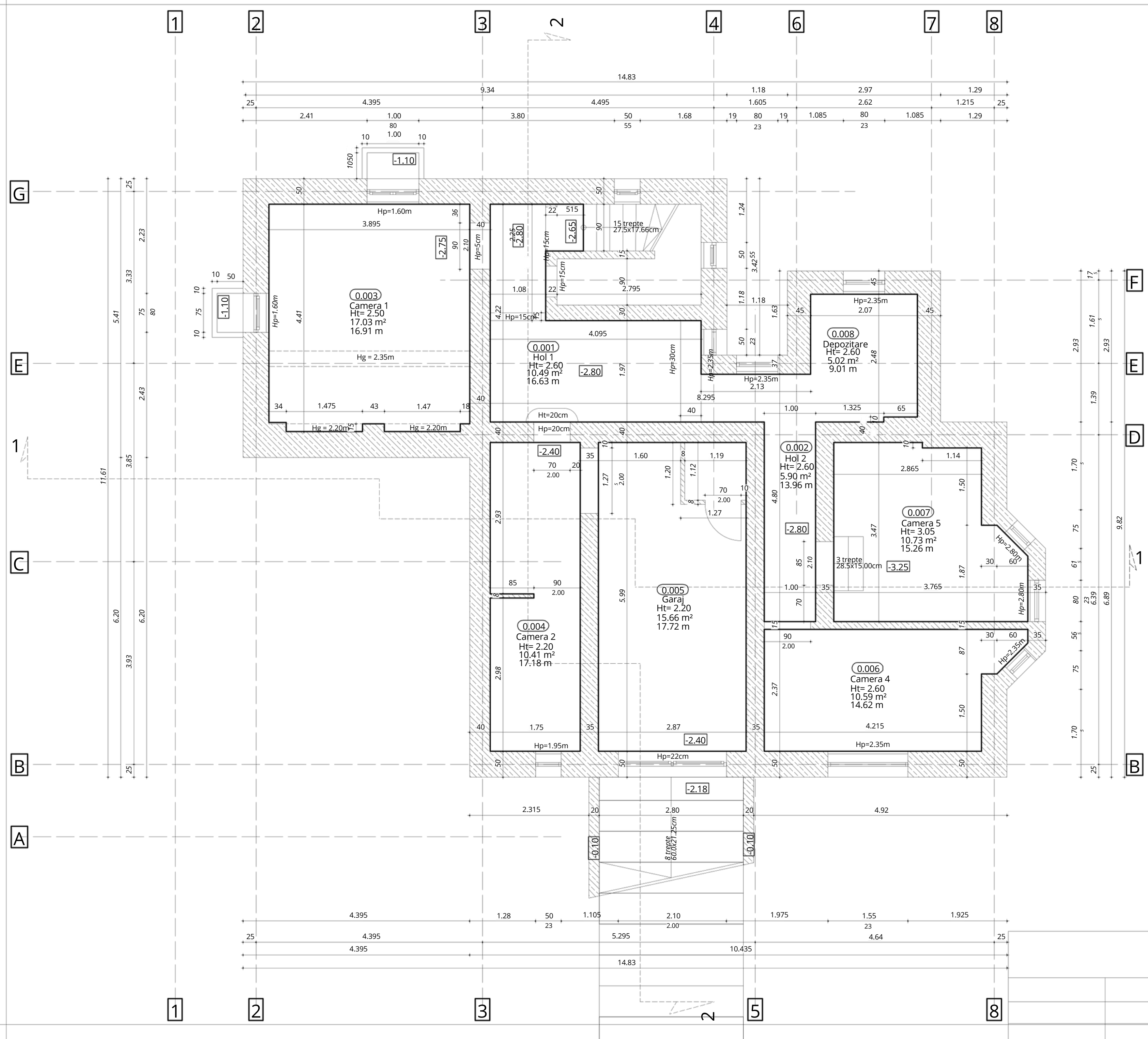
Plan Subsol
